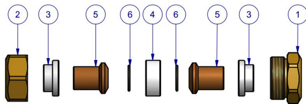
Exploded view
